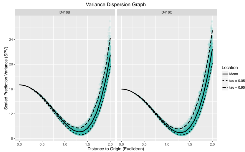
Figure 5: A VDG for Roquemore's hybrid designs D416B and D416C for a full quadratic model.
