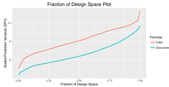
Figure 10: VDG for the D-optimal design of Goos and Jones (2011), for the two models.
