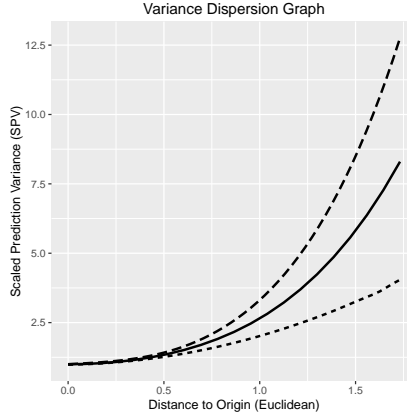
Figure 1: An example of a variance dispersion graph.
