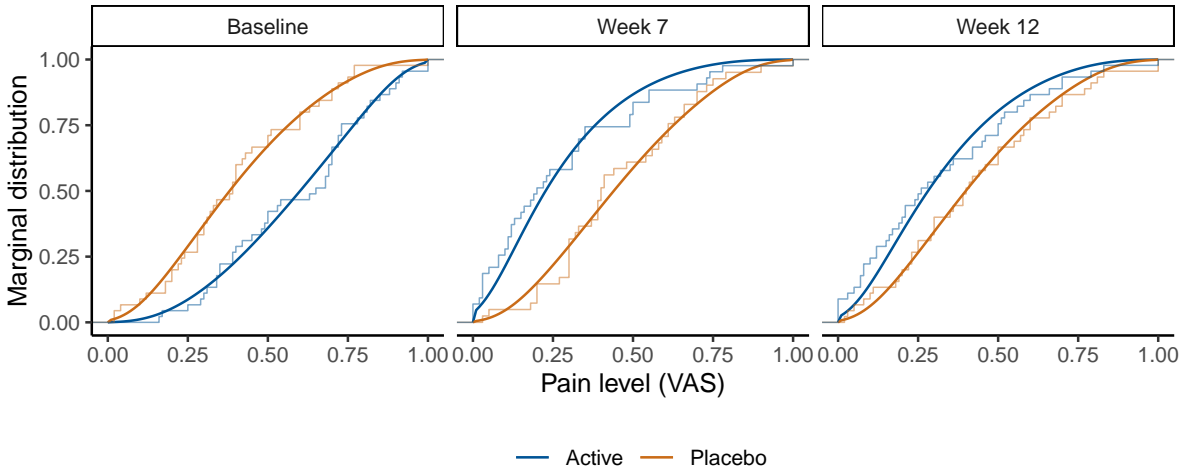
Figure 6: Comparison of marginal distributions, calculated from a mixed-effects continuous outcome logistic regression model, in the treatment (Active) and control (Placebo) groups at baseline and the two follow-up times. The step functions represent the empirical cumulative distribution functions of the specific groups.
