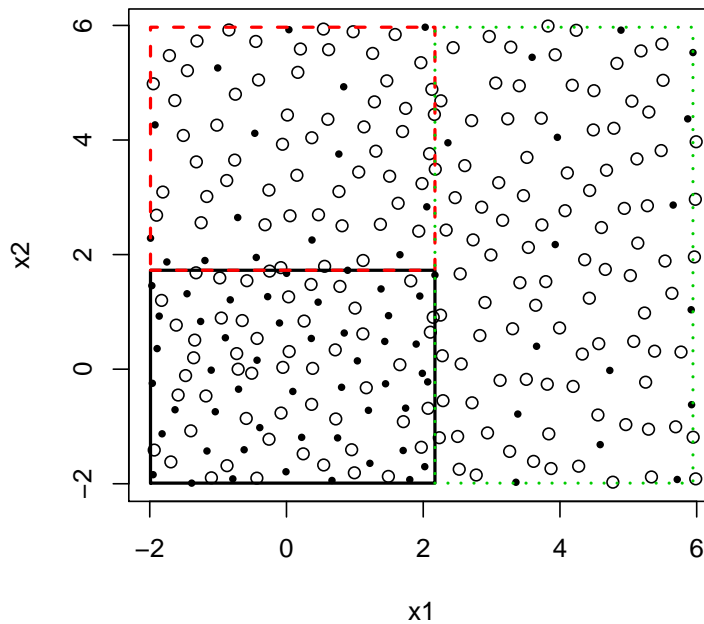
Figure 17: Treed D -optimal candidate locations XX (circles), input locations X (dots), and MAP tree \hat{\mathcal{T}}
