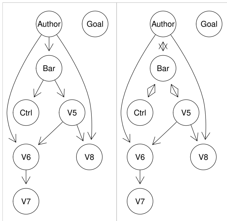
Figure 3: True underlying DAG (left) and CPDAG (right) estimated with the GES algorithm fitted on the simulated Gaussian dataset gmG8 .
