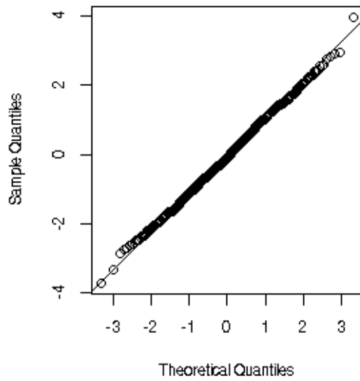
Normal Plot: Student (df=5) samples
