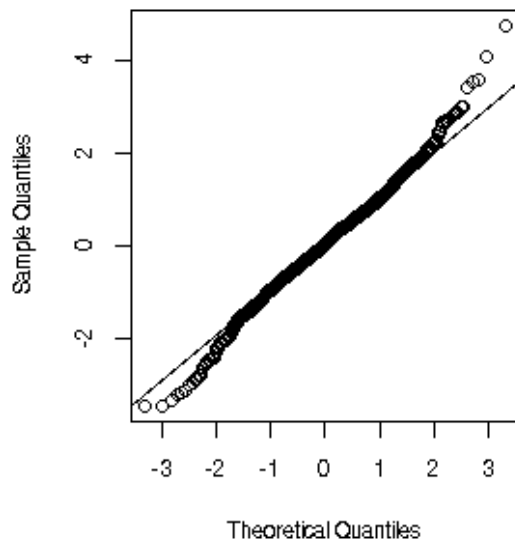
Normal Plot: Uniform samples
