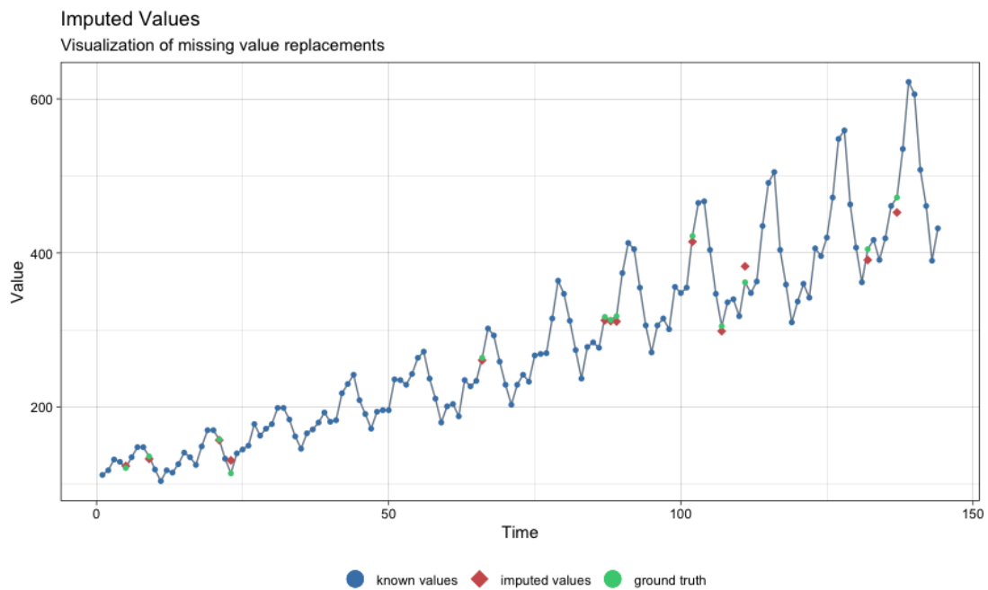
Figure 1: Results of imputation with na_kalman compared to real values
