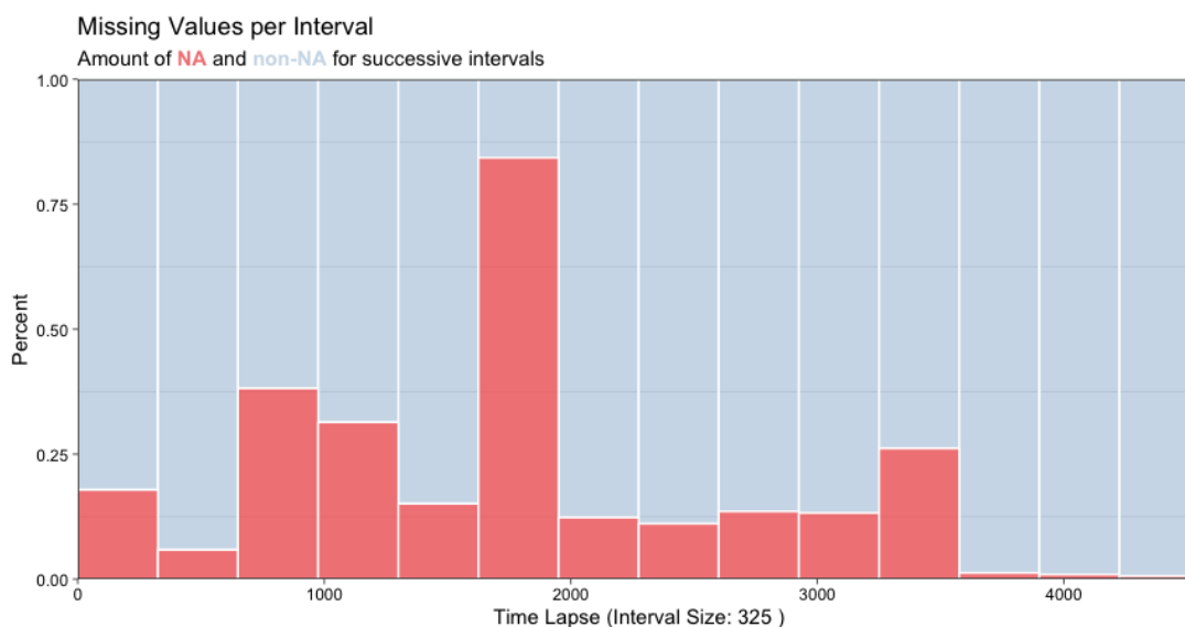
Figure 3: Example for ggplot_na_intervals
