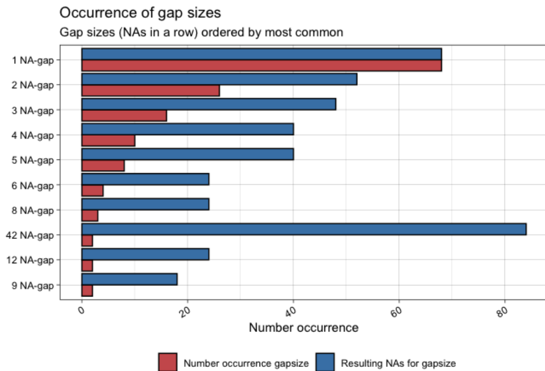
Figure 4: Example for ggplot_na_gapsize
