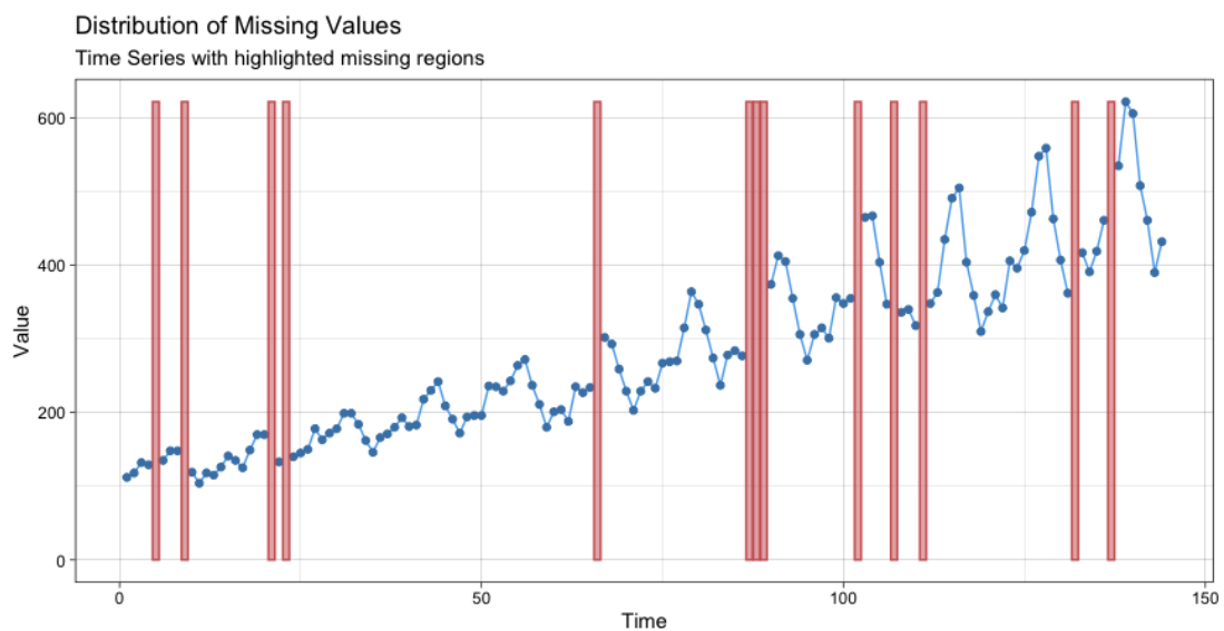
Figure 2: Example for ggplot_na_distribution
