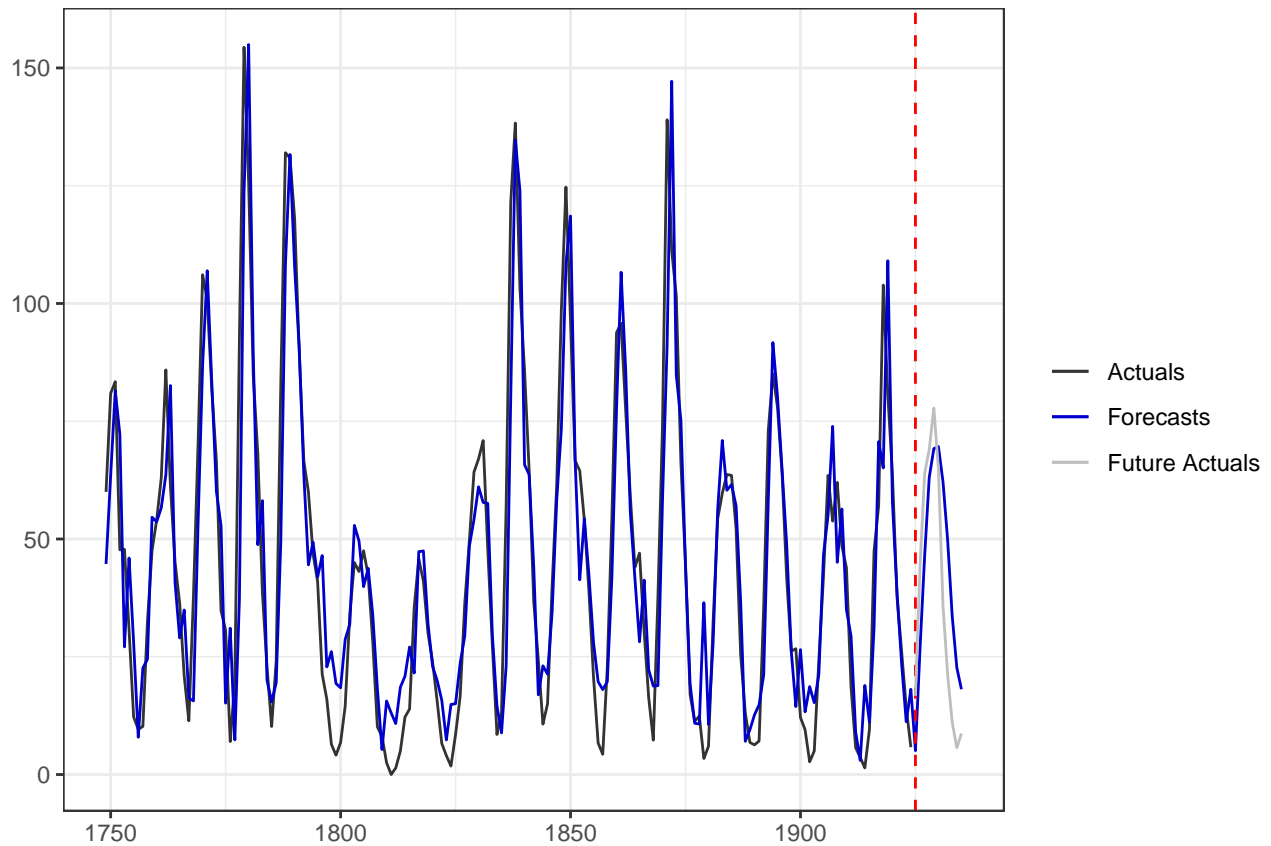
Sunspot Forecast using GARMA(8,0)
