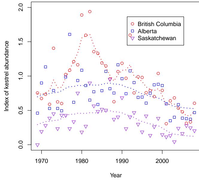
Fig. 15.4. Plot model 4 fits to the kestrel data.
