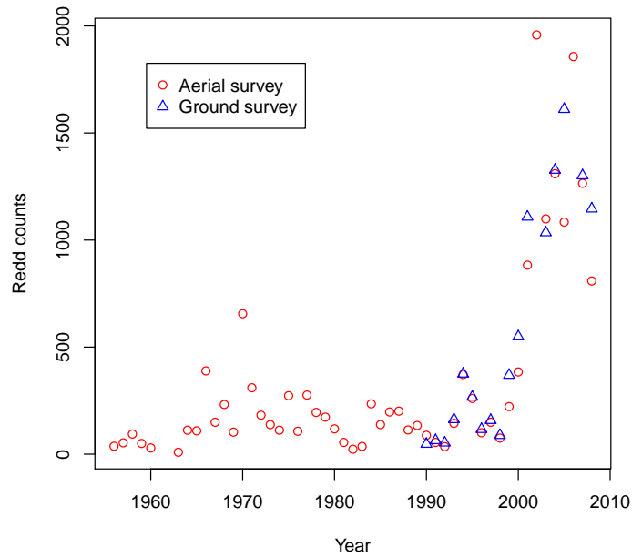
Fig. 15.1. The two time series look to be pretty close to one another in the years where there is overlap.
