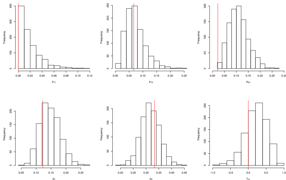
Figure 4: Posterior samples under the saturated model and a \text{Dir}(1,1,1,1,1,1,1,1) prior. MLEs are shown as vertical red lines.
