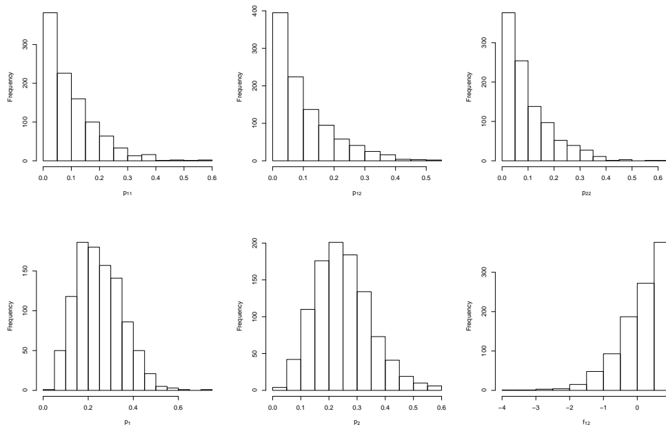
Figure 3: Prior samples under the saturated model and a \text{Dir}(1,1,1,1,1,1,1,1,1) prior.
