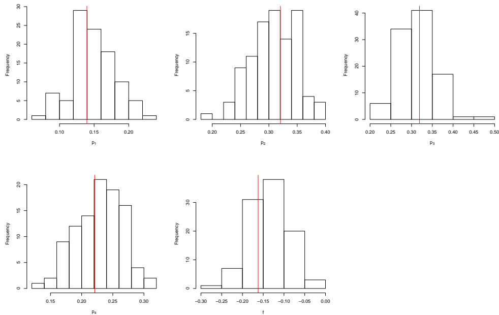
Figure 5: Posterior samples under the single f model. MLEs are shown as vertical red lines.
