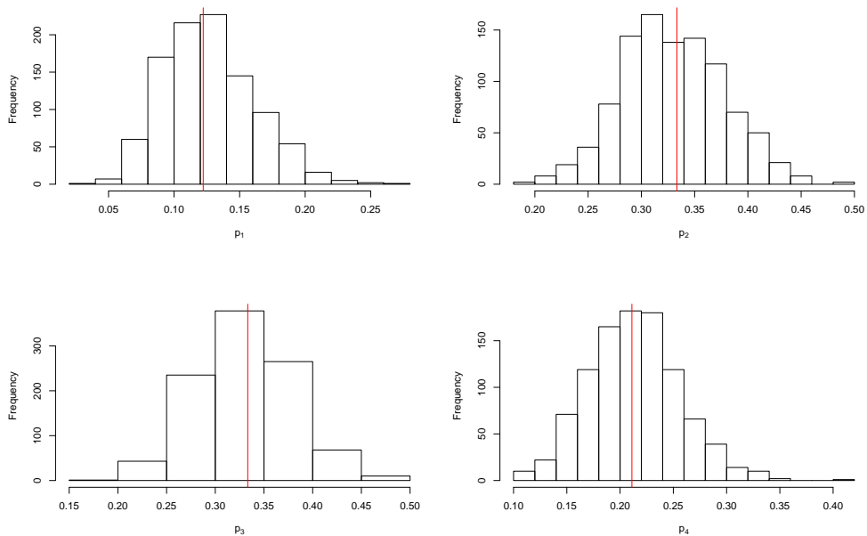
Figure 2: Posterior samples under HWE and a \text{Dir}(1,1,1,1) prior. MLEs are shown as vertical red lines.
