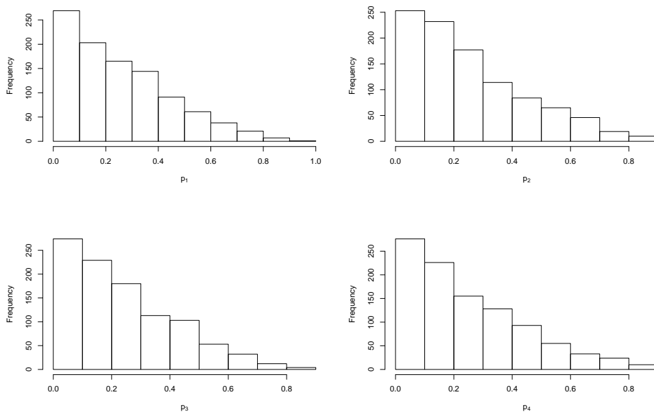
Figure 1: Samples from the prior \text{Dir}(1,1,1,1) under HWE.
