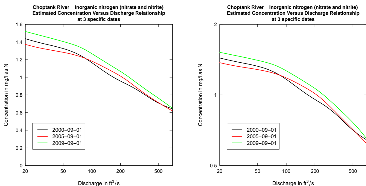
(a) plotConcQSmooth
