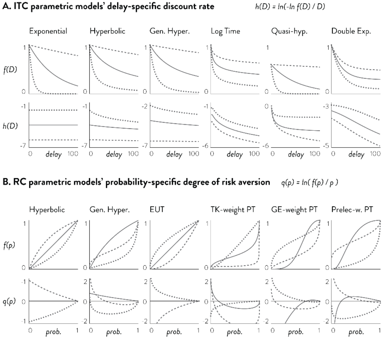
Figure 1. Parametric models' pattern of behavior. Each parametric model assumes a particular behavioral pattern. Shown in panel A is the delay-specific discount rate of ITC models in Table 1. All parametric models of ITC in consideration show either a constant (exponential) or decreasing delay-specific discount rates. Shown in panel B is the probability-specific degree of risk aversion, which is the log of the ratio between objective and subjective probabilities. A measure above 0 would indicate over-appreciation of probabilities and hence risk-seeking, while a measure below 0 would indicate risk-aversion. All parametric models of RC in consideration assume a behavioral pattern that switches between risk-aversion and risk-seeking at most once. In other words, probability-specific measure of risky choice for all RC parametric models can cross 0 (risk-neutral point) at most once.
