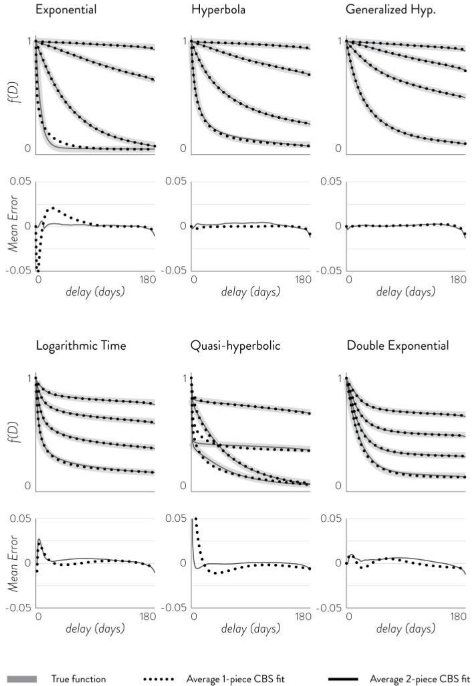
Supplemental Figure 3. Average CBS fits from ITC choice dataset simulation. CBS fits are shown overlaid on top of 6 different ITC utility functions. The first and the third row shows the true simulating utility functions and their average CBS fits. The average CBS fits were calculated by taking the mean of the 200 fitted CBS functions from the largest choice dataset (400 choices). The second and the fourth row shows the mean error of the fitted CBS functions and the true simulating functions.
