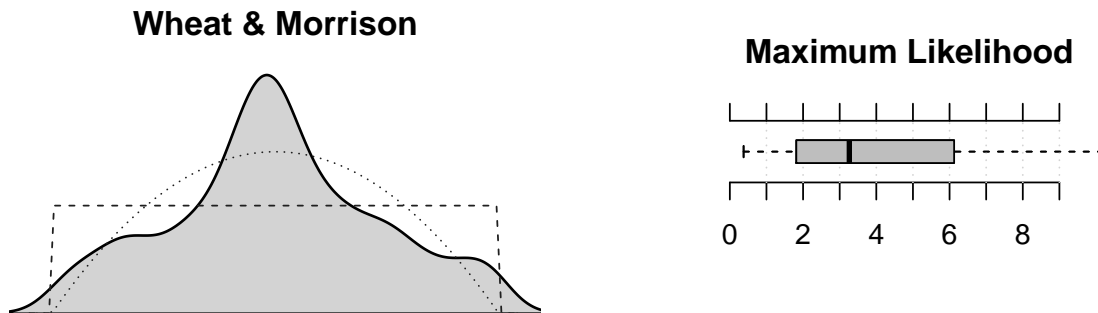
Figure 3: Diagnostic plots for estimating regularity
