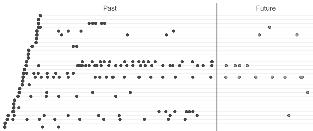
Figure 1: Timing patterns for sampled grocery customers
