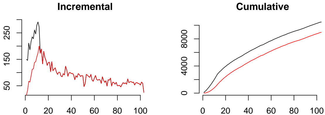
Figure 2: Weekly trends for the grocery dataset
