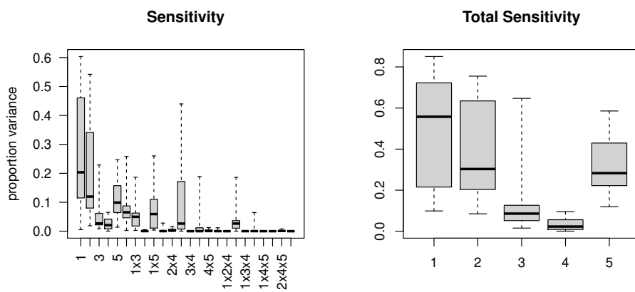
Figure 21: Sobol decomposition - air foil data.
