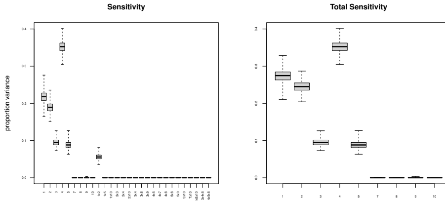
Figure 6: BASS sensitivity analysis - Friedman function.
