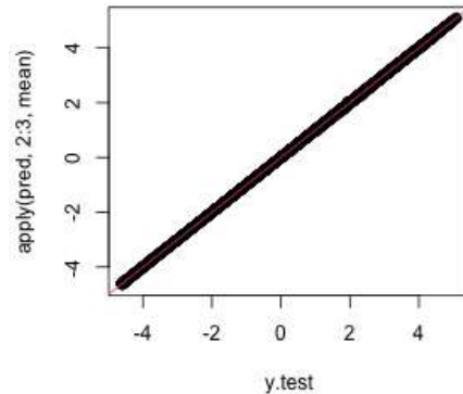
Figure 22: BASS prediction performance - pollutant spill model.
