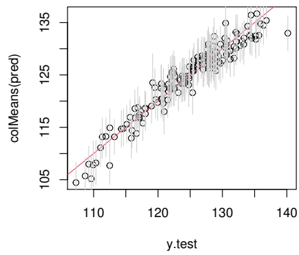
Figure 20: Prediction performance - air foil data.
