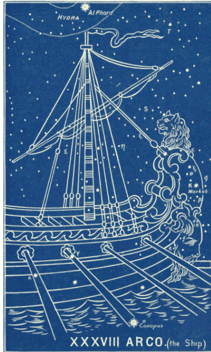
Plate 38: ARGO (the Ship)
