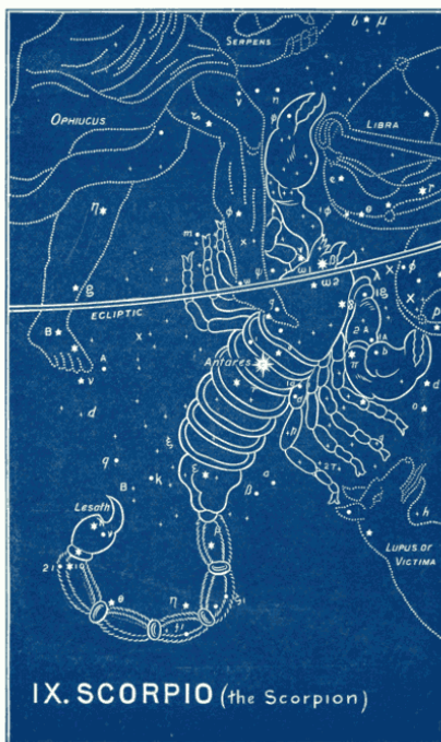
Plate 9: SCORPIO (the Scorpion)
