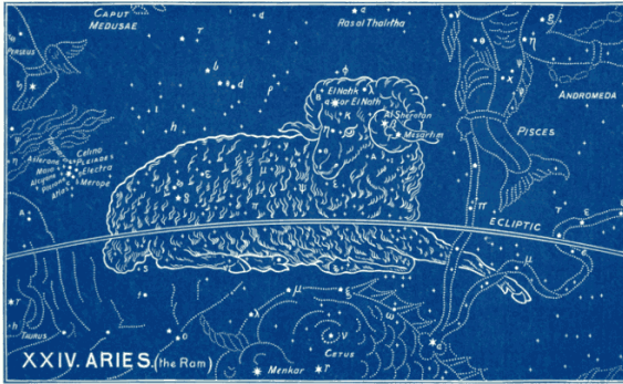
Plate 24: ARIES (the Ram)
