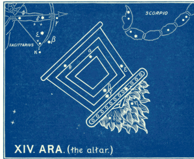
Plate 14: ARA (the Altar)
