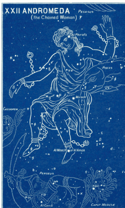
Plate 22: ANDROMEDA (the Chained Woman)
