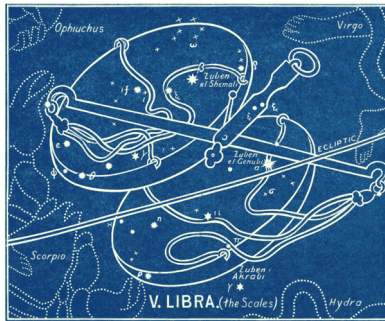
Plate 5: Libra (the Scales)
