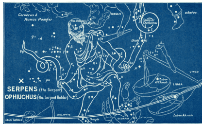
Plate 10: SERPENS (the Serpent) and OPHIUCHUS (the Serpent Holder)
