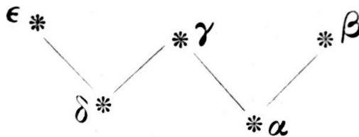
Illustration showing the W of Cassiopeia
