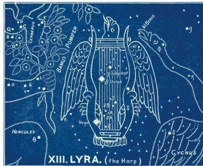
Plate 13: LYRA (the Harp)
