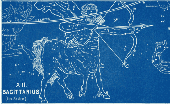
Plate 12: SAGITTARIUS (the Archer)
