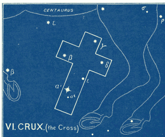
Plate 6: Crux (the Cross)
